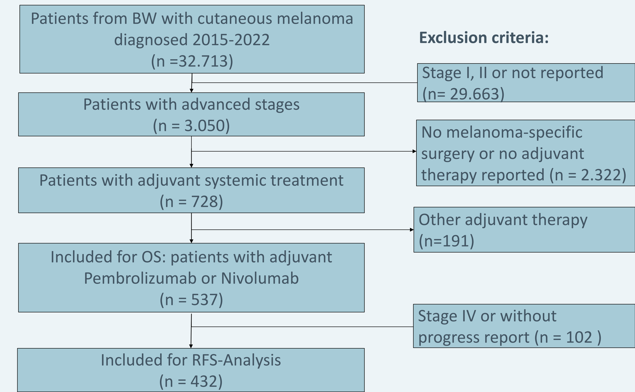
Fig. 1: Consort Diagram
